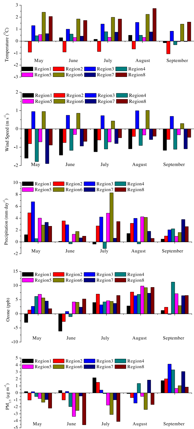
Fig. 4. Monthly-mean MBs of temperature at 2-m, wind speed at 10-m, daily total precipitation, and concentrations of max 8-h average O 3 and 24-h average PM 2.5 in different regions (see definition of regions 1–8 in Fig. 2) for May–September 2009.
