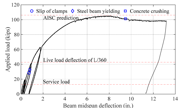
Figure 4: Load-deflection curve of Specimen 1
