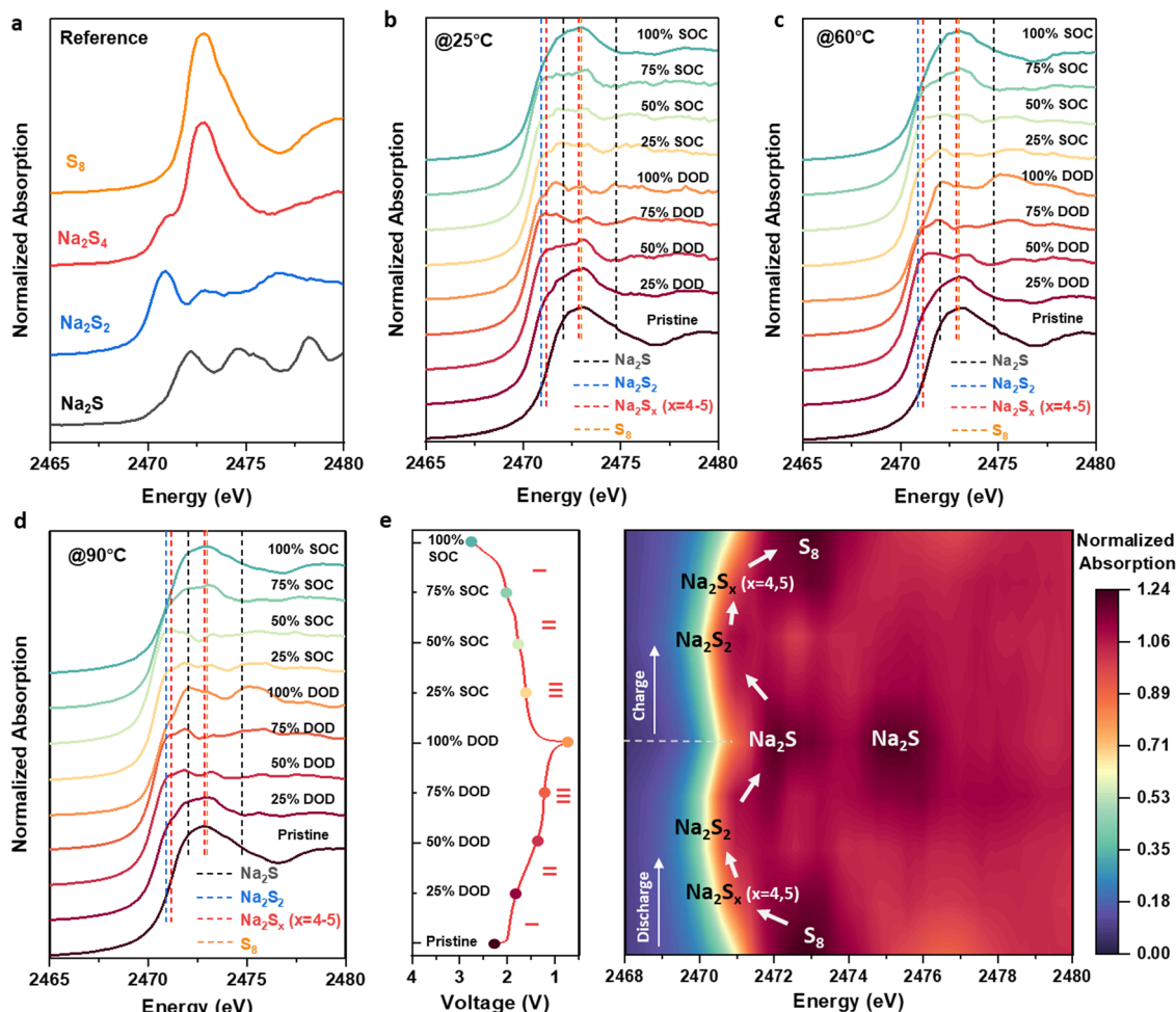
Fig. 4 Ex situ X-ray absorption spectroscopy (XAS) investigation of ASSSBs. (a) S K-edge XANES spectra of Na 2 S, Na 2 S 2 , Na 2 S 4 , and S. Ex situ S K-edge XANES measurements for the ASSSBs operated at (b) 25 °C, (c) 60 °C, and (d) 90 °C. (e) The voltage profile and intensity mapping of the ex situ S K-edge XANES of the cell operated at 90 °C.
